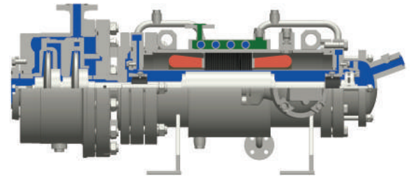
CANNED MOTOR PUMPS OF CMP SERIES
